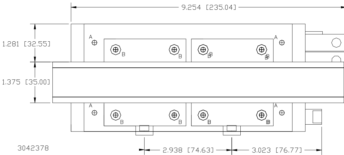
FIGURE 4. RKW 600W POWER SUPPLY WITH KIT INSTALLED, OUTLINE DIMENSIONS
